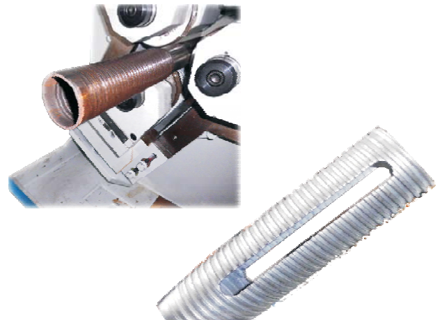
PIPE THREAD ROLLING MACHINE
